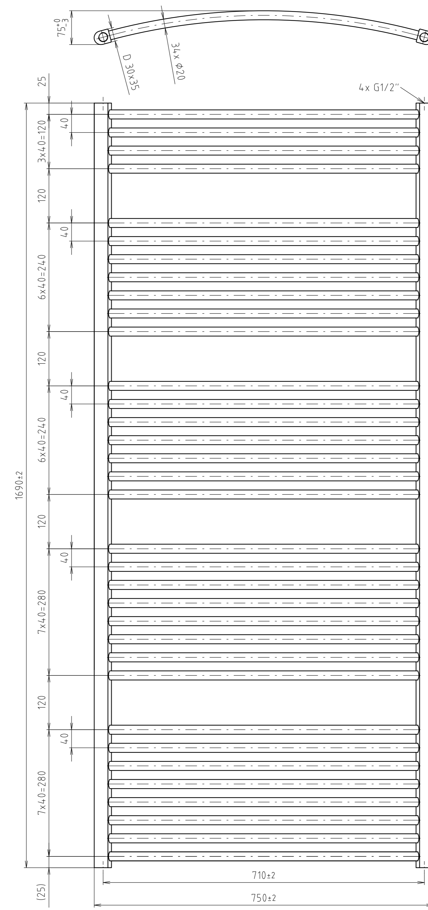
GRANDE RADIUS 1690/750
