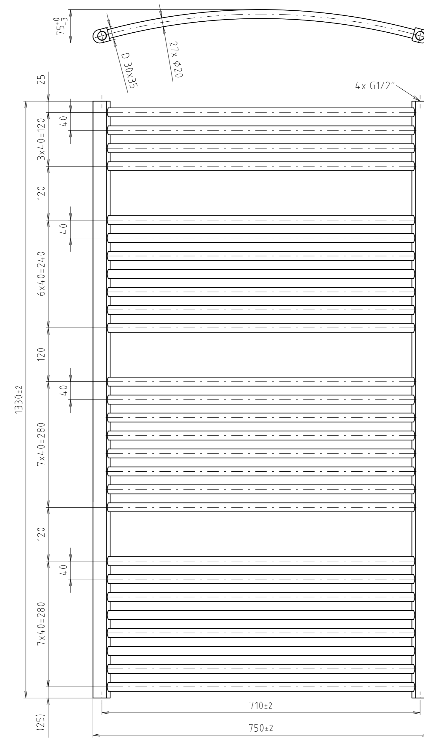
GRANDE RADIUS 1330/750
