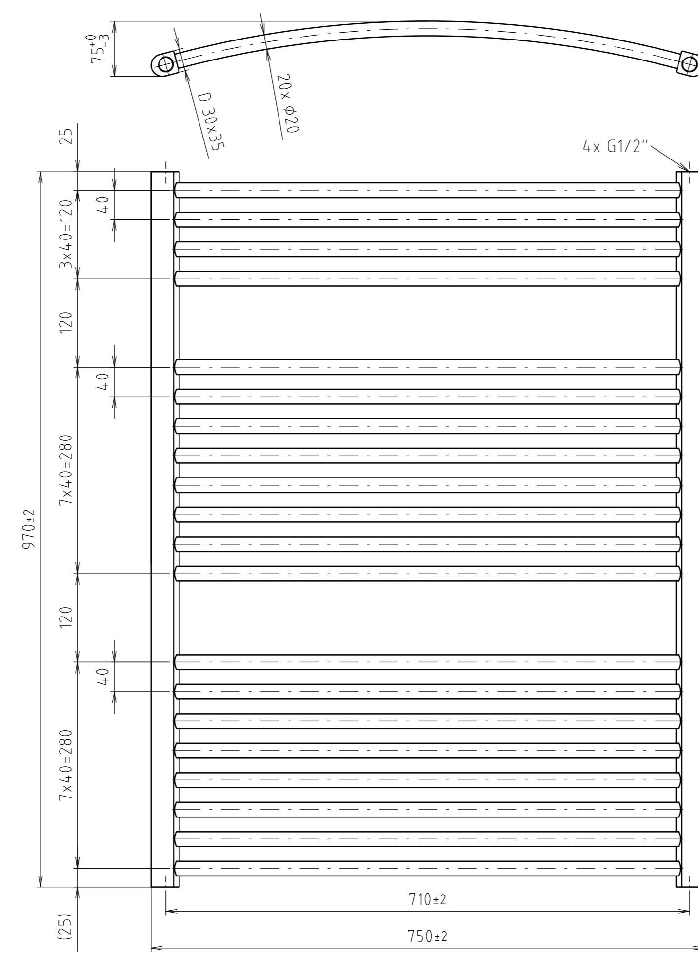
GRANDE RADIUS 970/750
