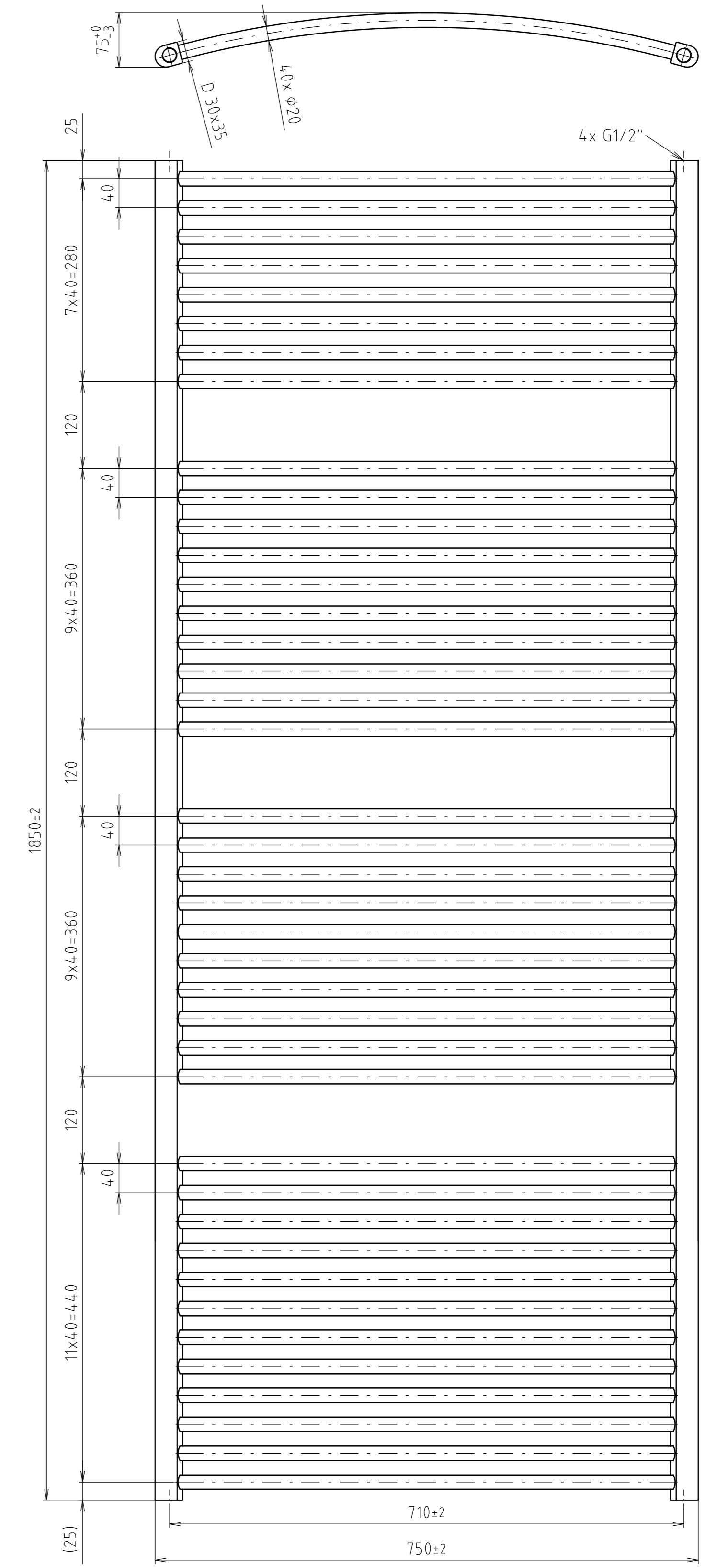
GRANDE RADIUS 1850/750
