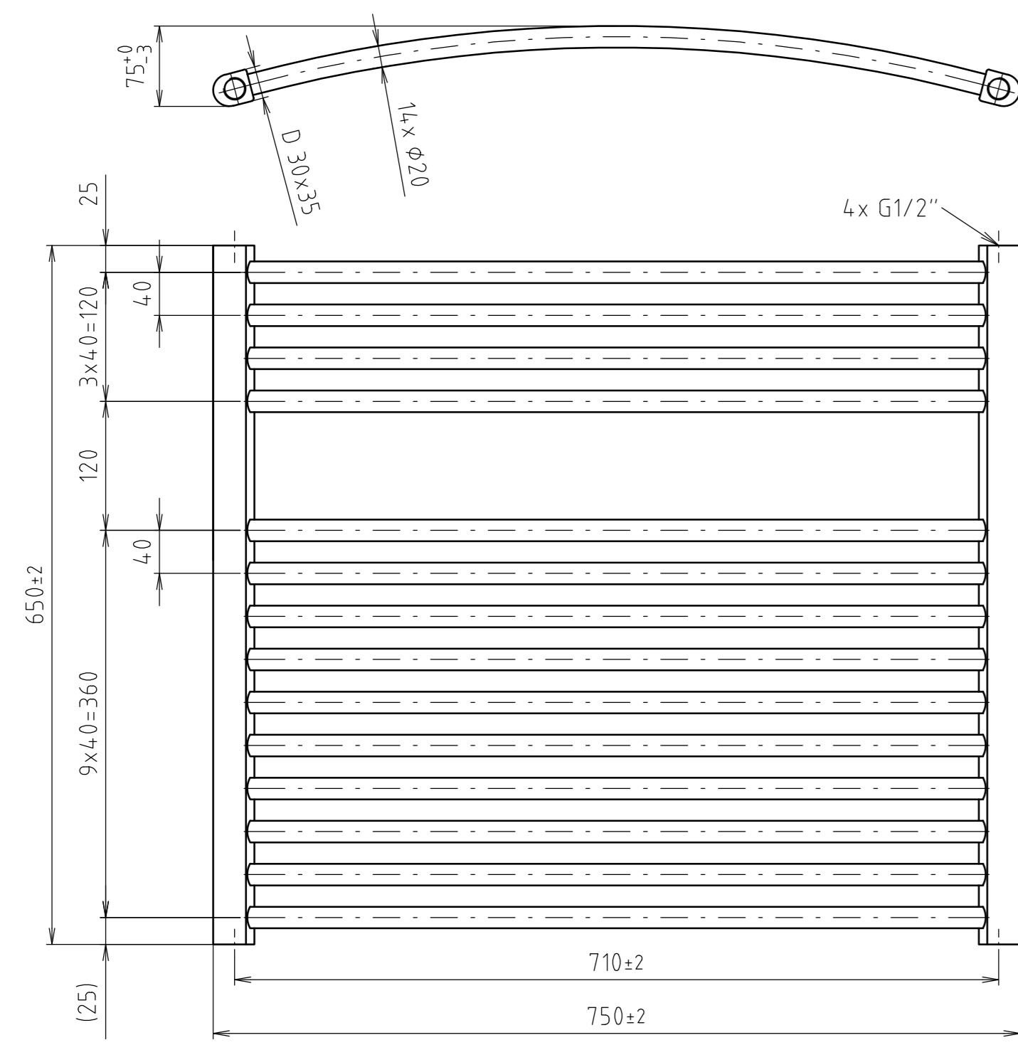
GRANDE RADIUS 650/750
